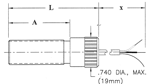
0018 5/8-18 SHOWN WITH SHIELDED CABLE "LSx"
