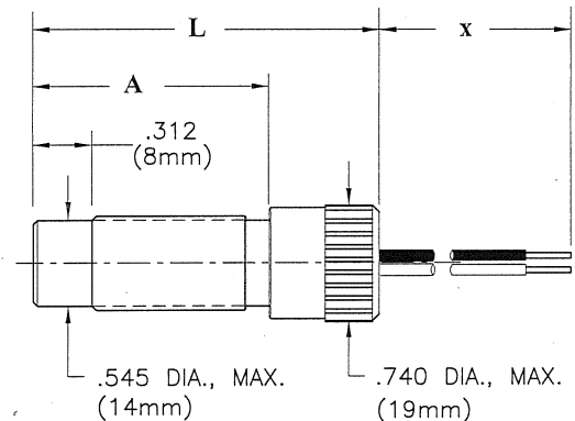
0018 5/8-18 SHOWN WITH SHIELDED CABLE "LSx"
