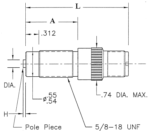
0018B 5/8-18 SHOWN WITH SHIELDED CABLE "Lx"
